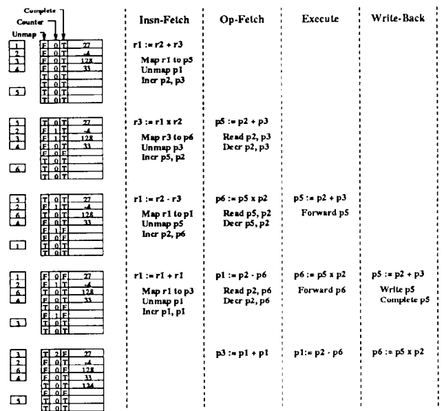
Figure 4: Reclaiming Registers
