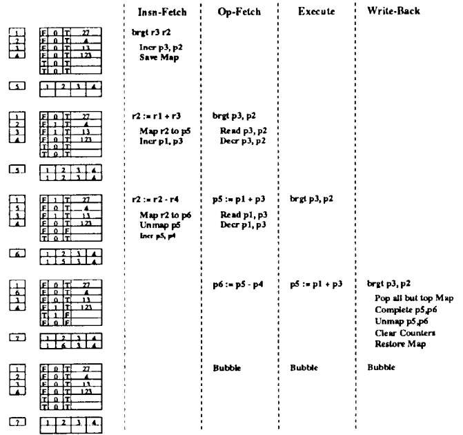
Figure 6: Mispredicted Branch
